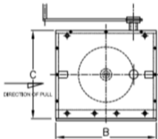
VIEW B-B
